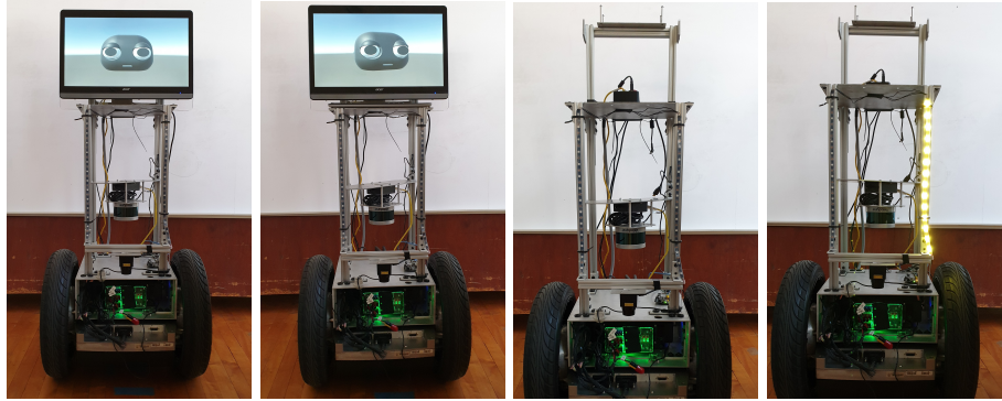
Fig. 4. Gaze and LED Signals. From left to right: Neutral gaze; Gaze signaling to the left lane; Neutral LED; LED blinking to signal a move to the left lane.
